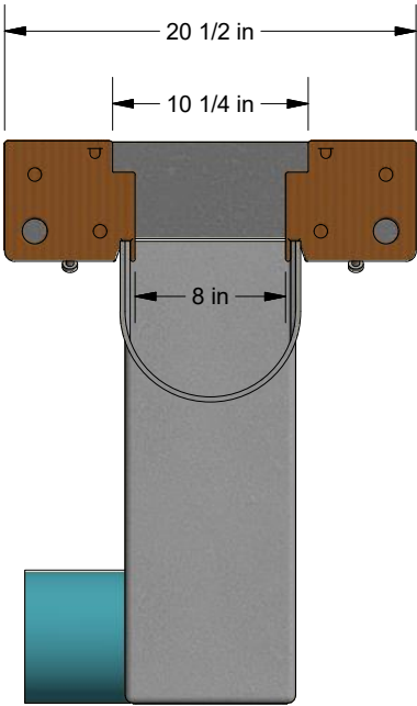
END VIEW
