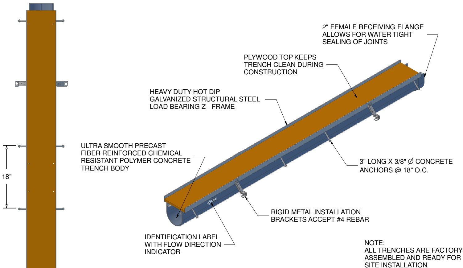
ISOMETRIC VIEW
