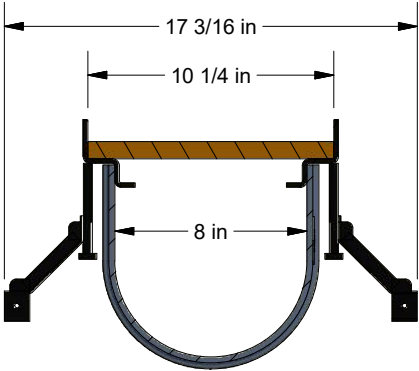
SECTION A-A SCALE 1:8
