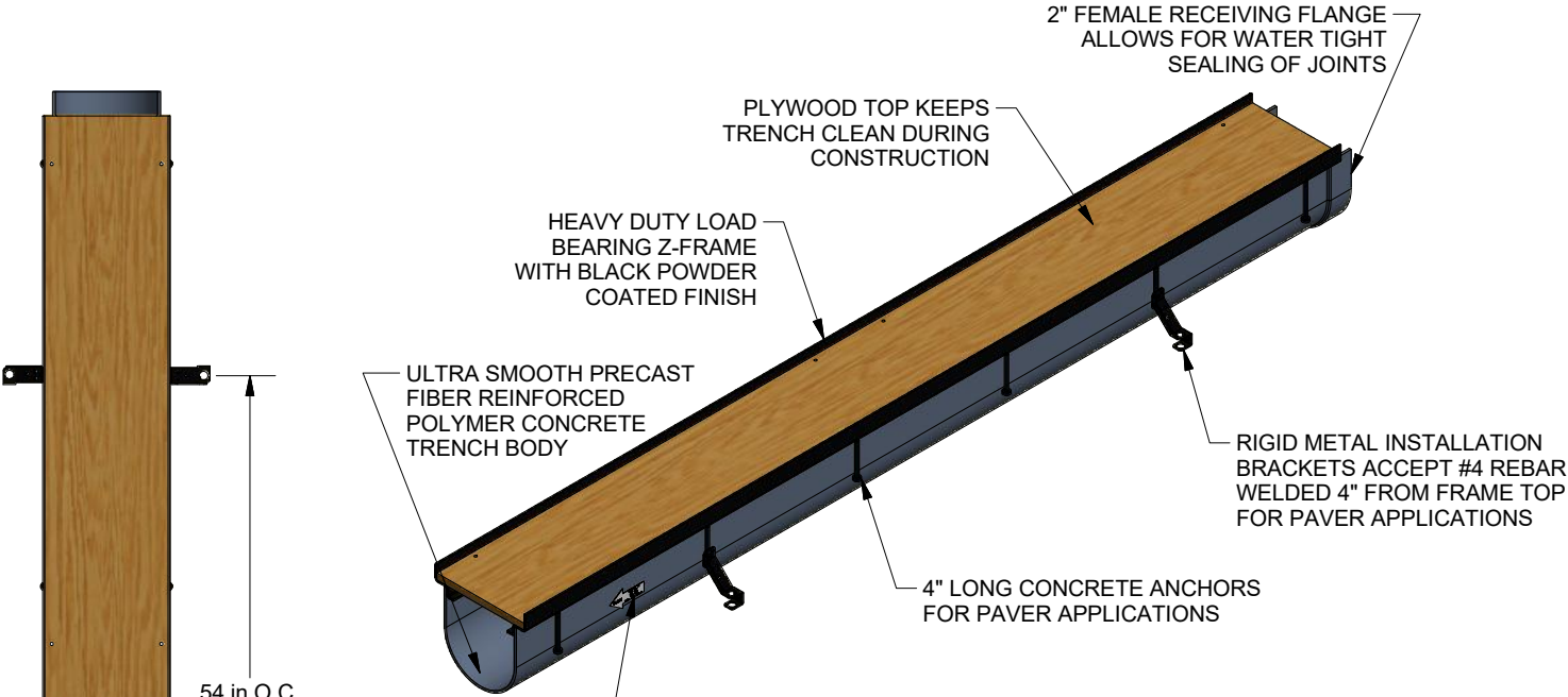
ISOMETRIC VIEW
