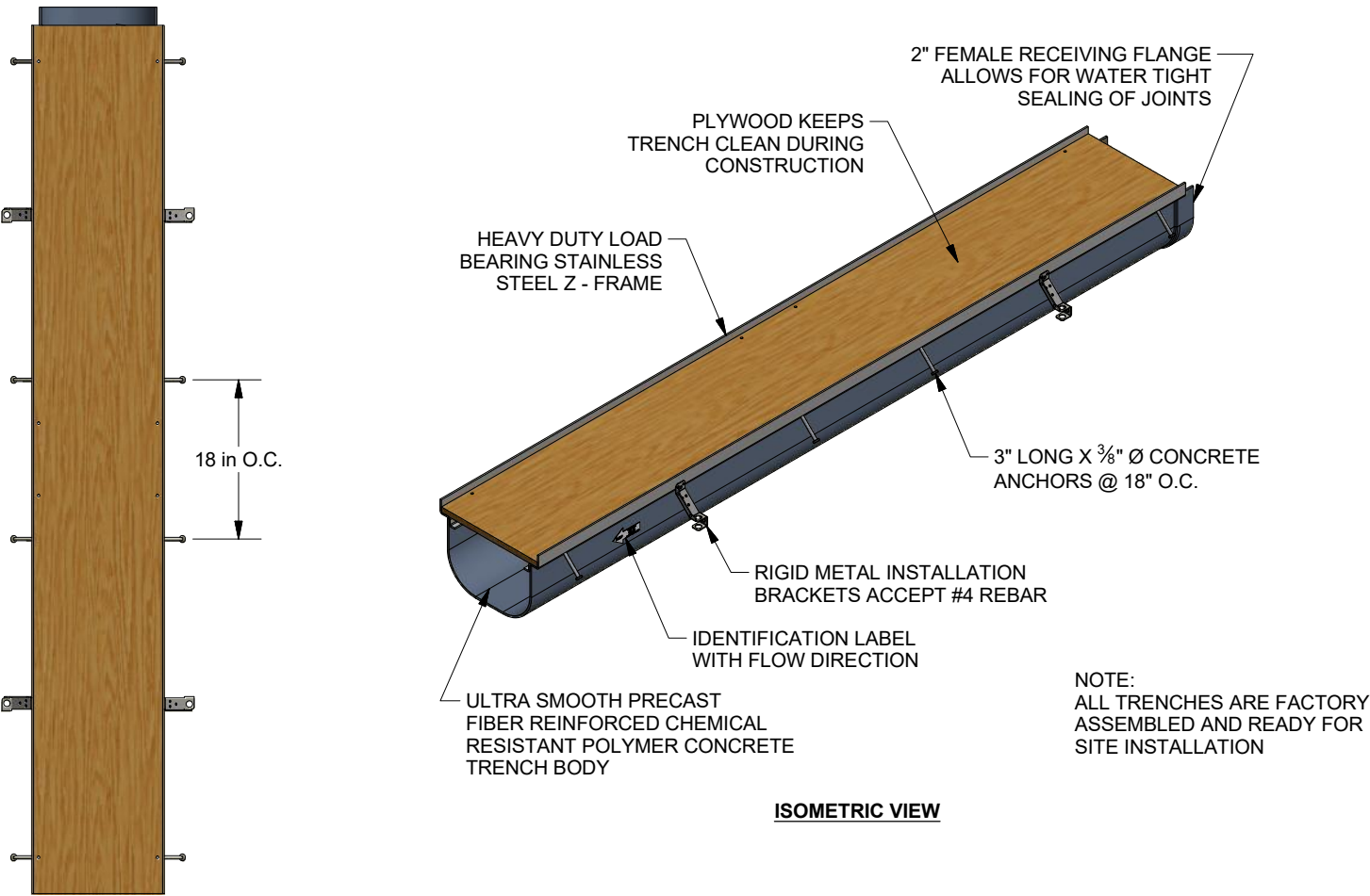
TOP VIEW
