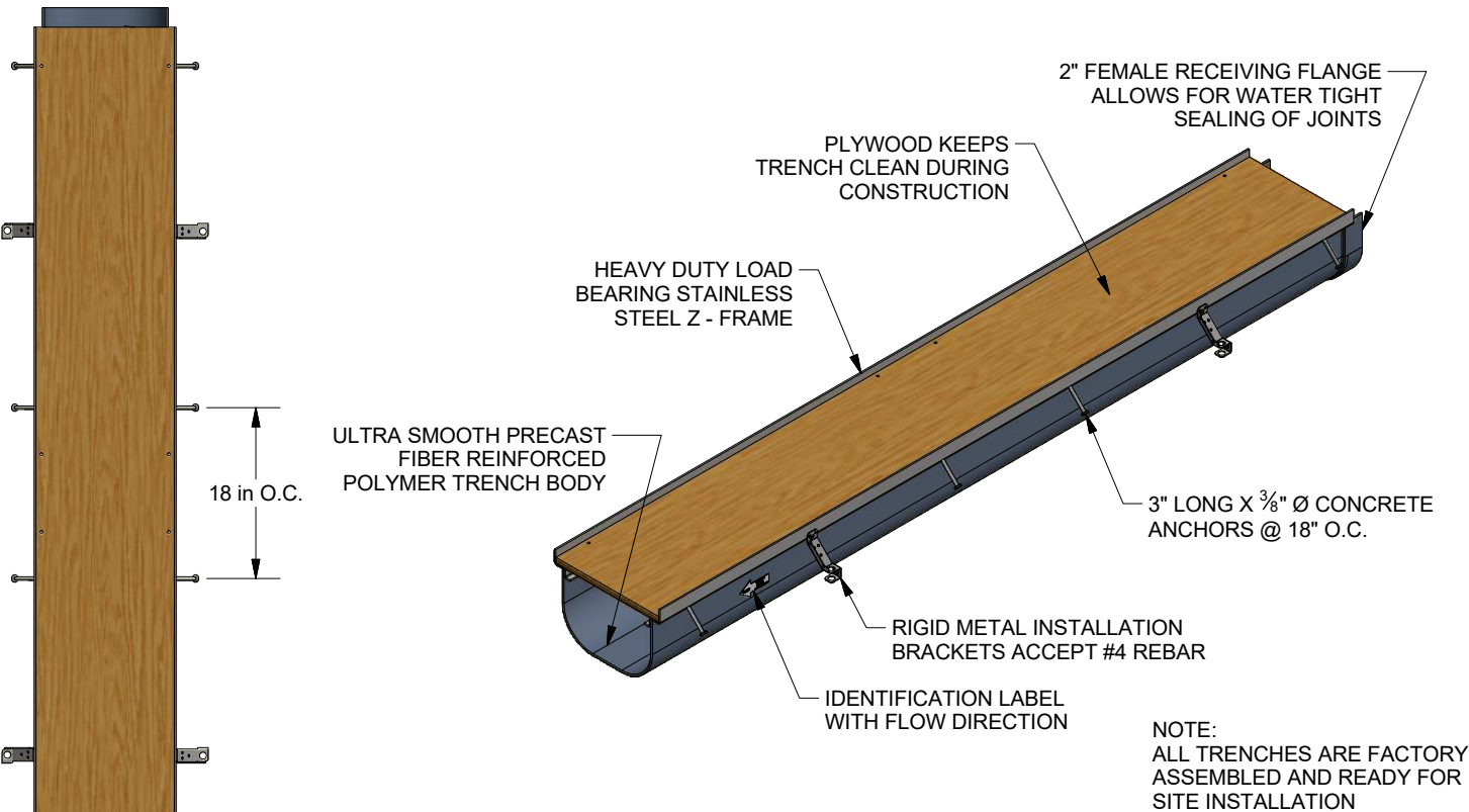
ISOMETRIC VIEW
